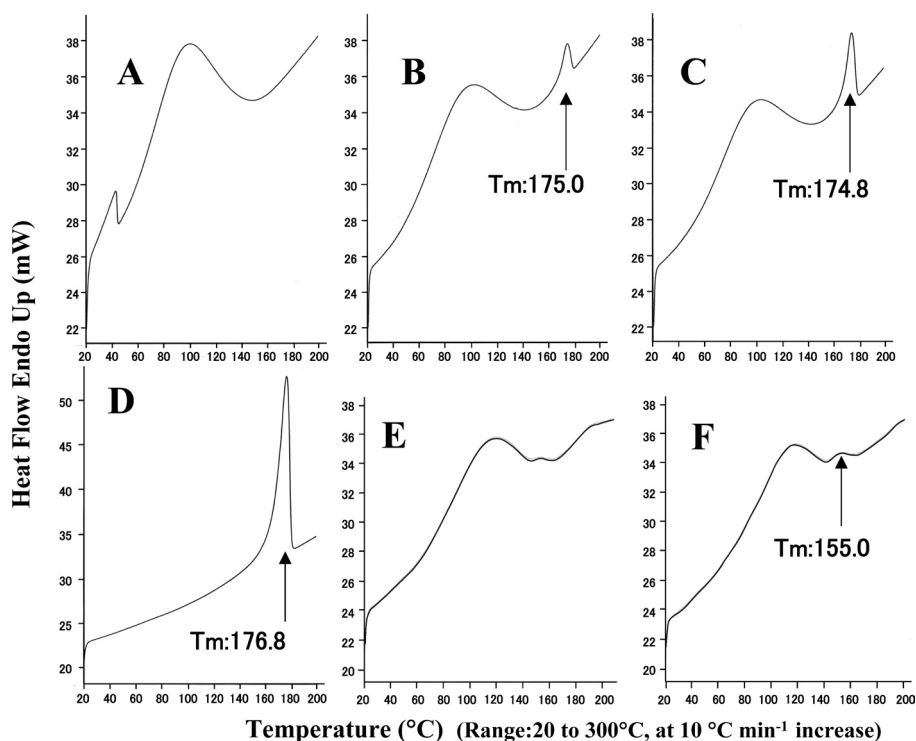
Figure 7. DSC measurements for cellulose (A), a 10% PHB blend (B), a 20% PHB blend (C), 100% PHB (D), non-transformed rice (E), and transformed rice (F).
